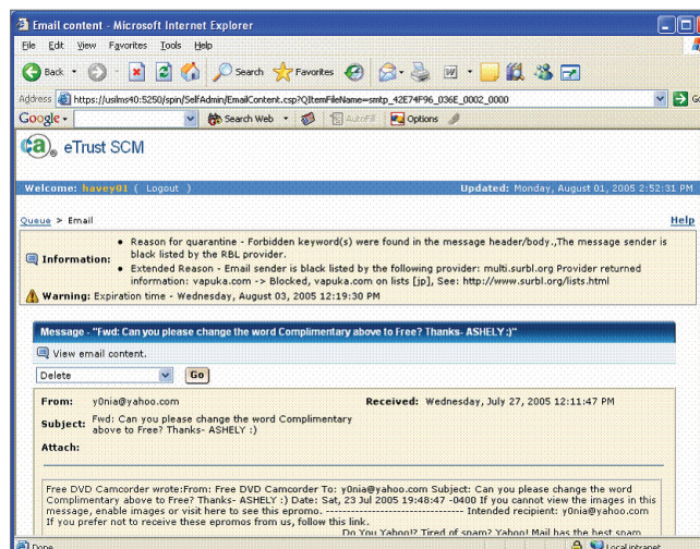
Figure 2. Web-based interface enables users to search and manage quarantined emails in real time.
